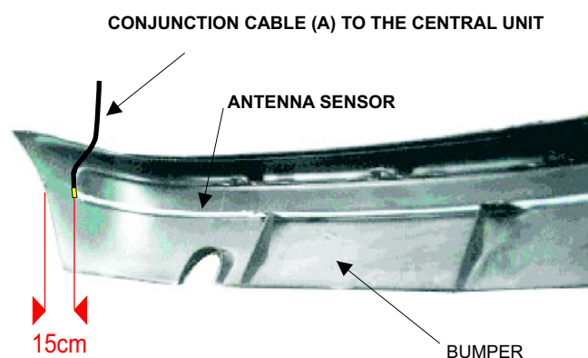
Fig.1 - Sight of antenna assemblage inside bumper
